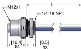
Female Receptacles
