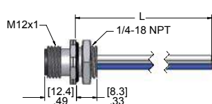
Male Receptacles
