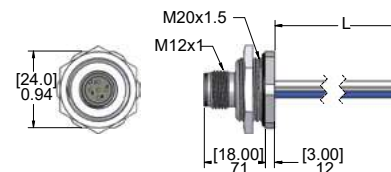
Male Receptacle
