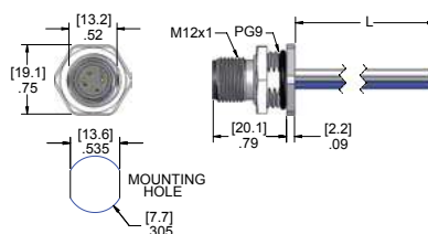
Male Receptacle
