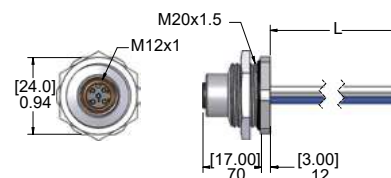
Female Receptacle
