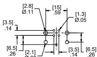
4 Pole Male Straight Layout
