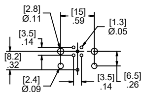
5 Pole Male Straight Layout
