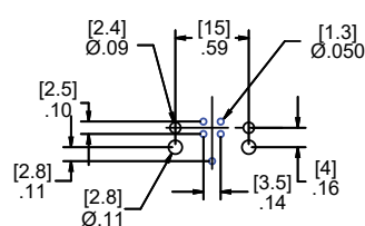
4 Pole Male Right Angle Layout
