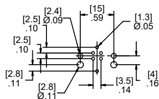
5 Pole Male Right Angle Layout
