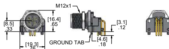
Male Right Angle
