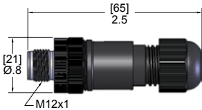
Male Plugs
