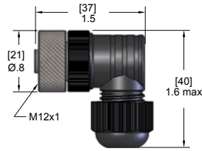
Female Plugs
