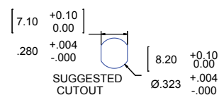
Male Receptacle
