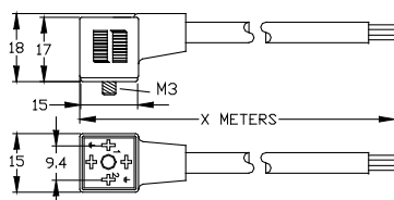
2 Poles + Ground (Dual Ground)
