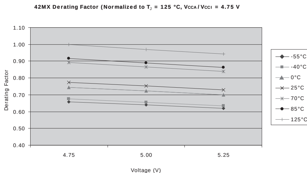
Figure 31 • 42MX Junction Temperature and Voltage Derating Curves (Normalized to T_J = 125^\circ\text{C} , V_{CCA}/V_{CCI} = 4.75\text{ V} )
