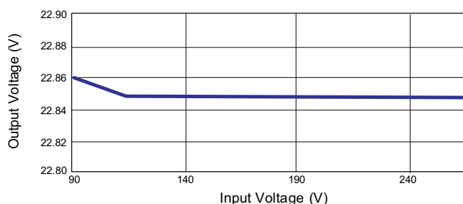
Fig.1 Line Regulation of Output Voltage
