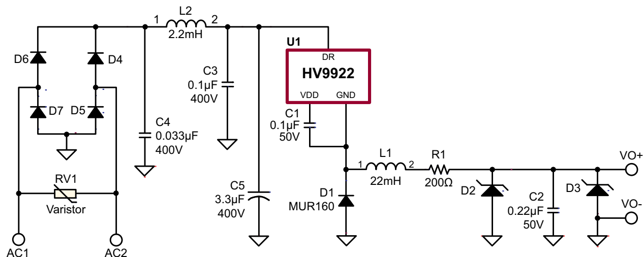
Circuit Schematic:
