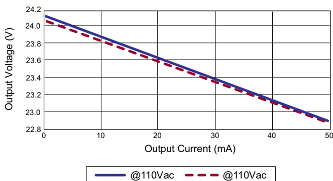
Fig.2 Load Regulation of Output Voltage
