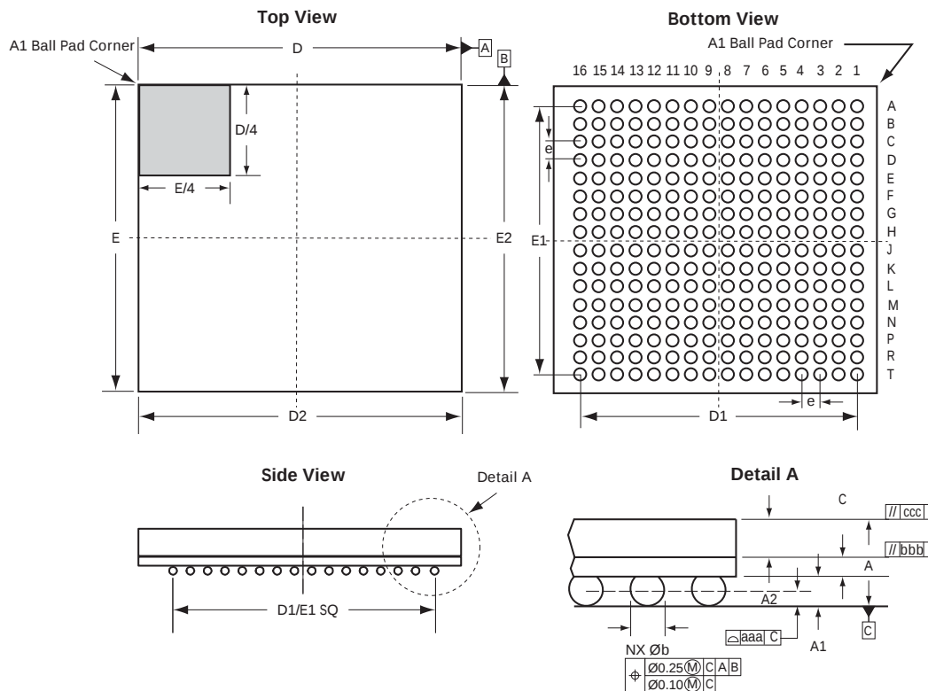
Figure 43 • Package Outline of FG256 MO-192 VAR DAF1
