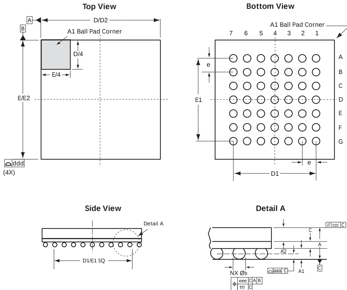
Figure 57 • Package Outline of CS49
