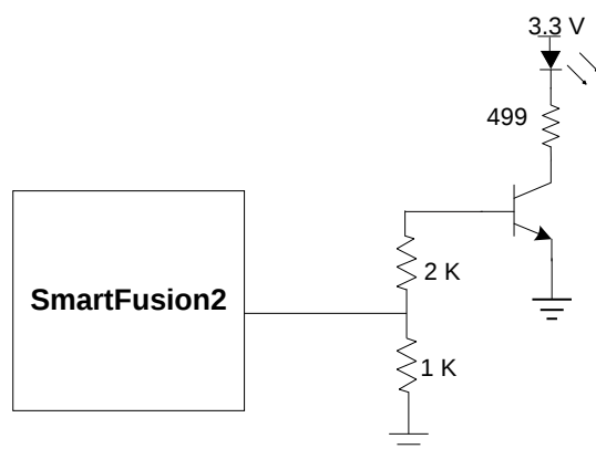
Figure 17 · LEDs Interface
