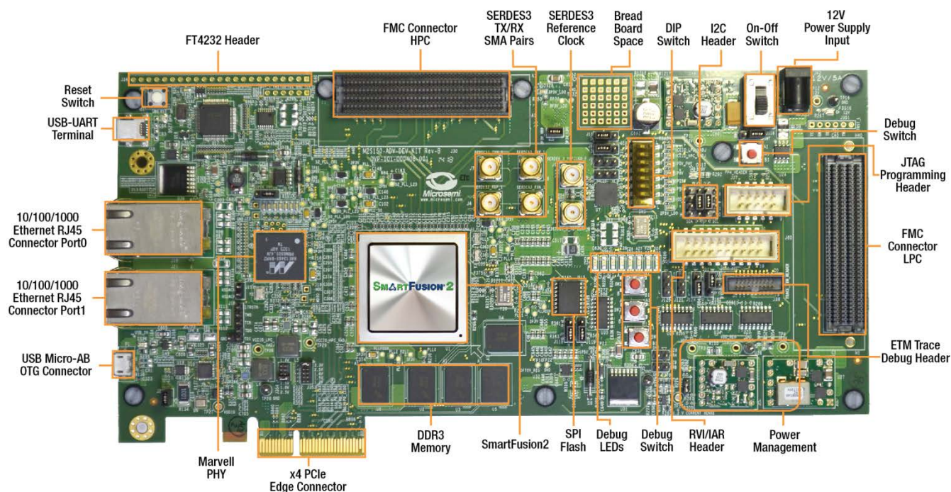
Figure 2 · SmartFusion2 Advanced Development Kit Board
