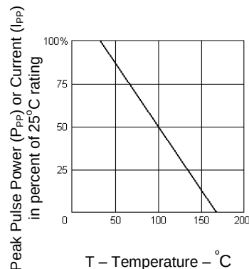
FIGURE 3 Derating curve
