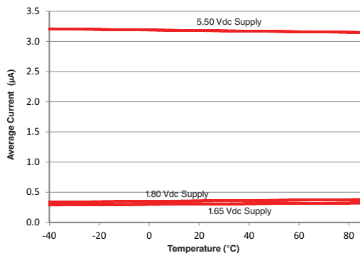
Figure 4. SM353LT Typical Performance Characteristics
