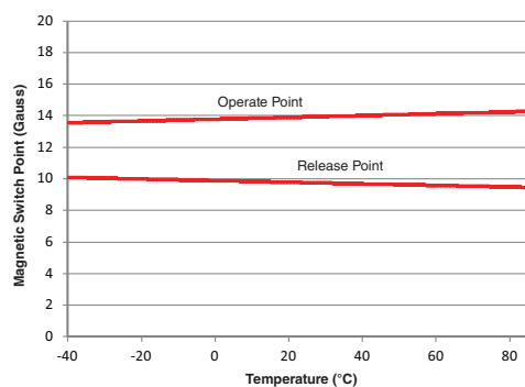
Figure 4. SM353LT Typical Performance Characteristics
