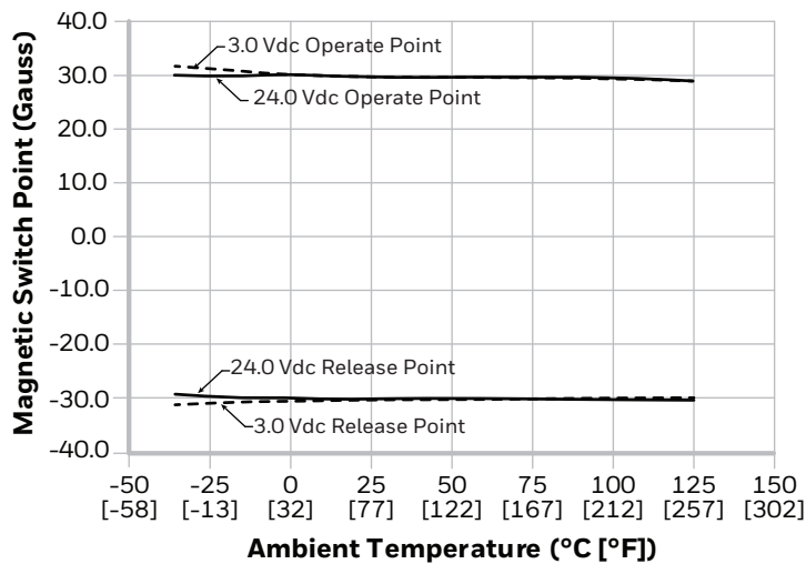
Figure 4. Magnetic Activation
