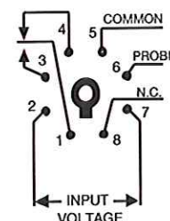
PIN CONFIGURATION DWG4787/9/93
