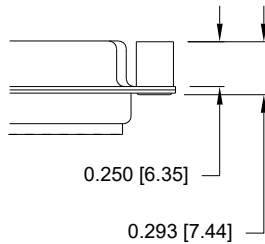
03 ..... 0.250" (MATING SIDE)
