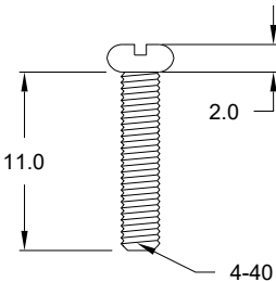
HOUSING SCREW
