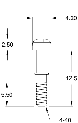
MATING SCREW
