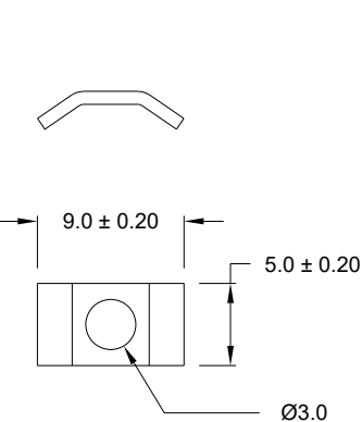
SADDLE WASHER
