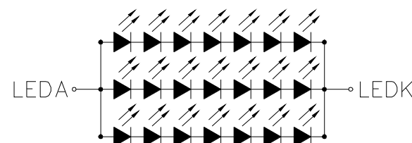
CONSTANT CURRENT: 60mA BACKLIGHT DRIVER CIRCUIT DIAGRAM
