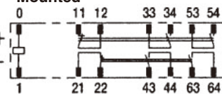
G7SA-4A2B Mounted
