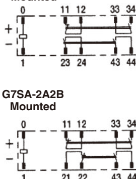
G7SA-3A1B Mounted
