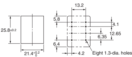
Mounting Holes and PCB Cutout Dimensions
