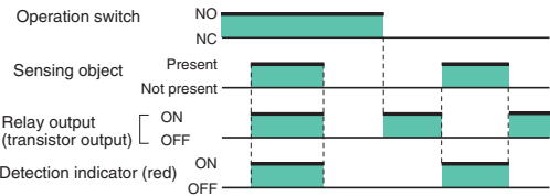
Timing Chart
