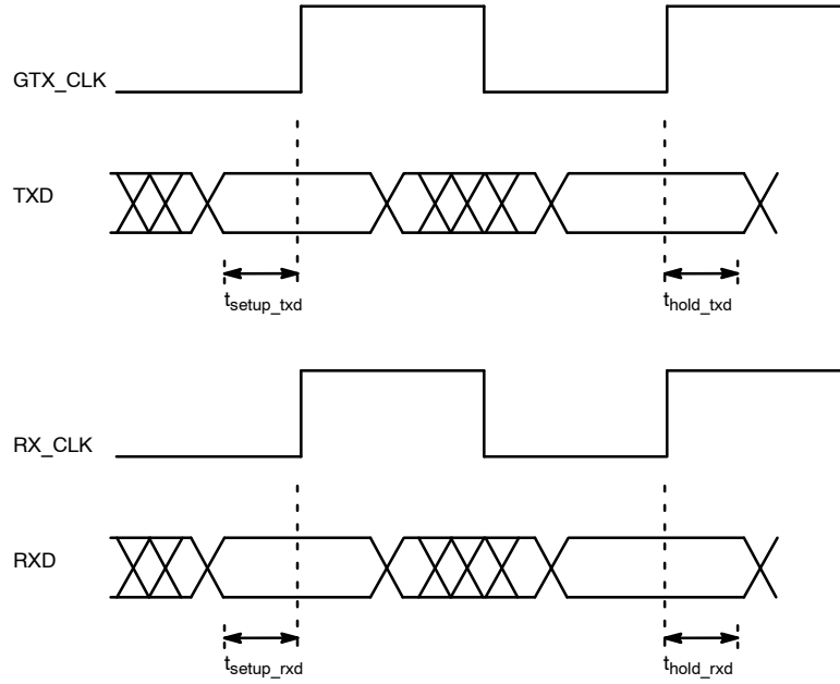
Figure 15. GMII I/O Timing Diagram
