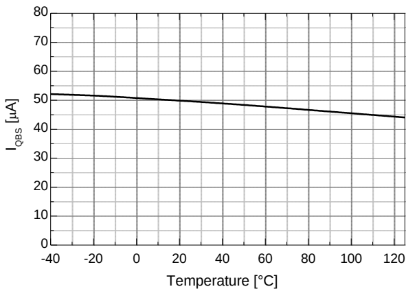
Figure 14 Quiescent V_{BS} Supply Current vs. Temperature
