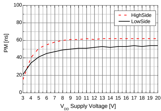
Figure 36 Output Pulse-Width Matching vs. VDD Supply Voltage
