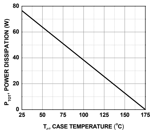
Figure 4. Power Derating
