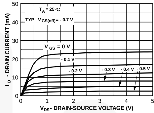
Figure 2. Common Drain-Source
