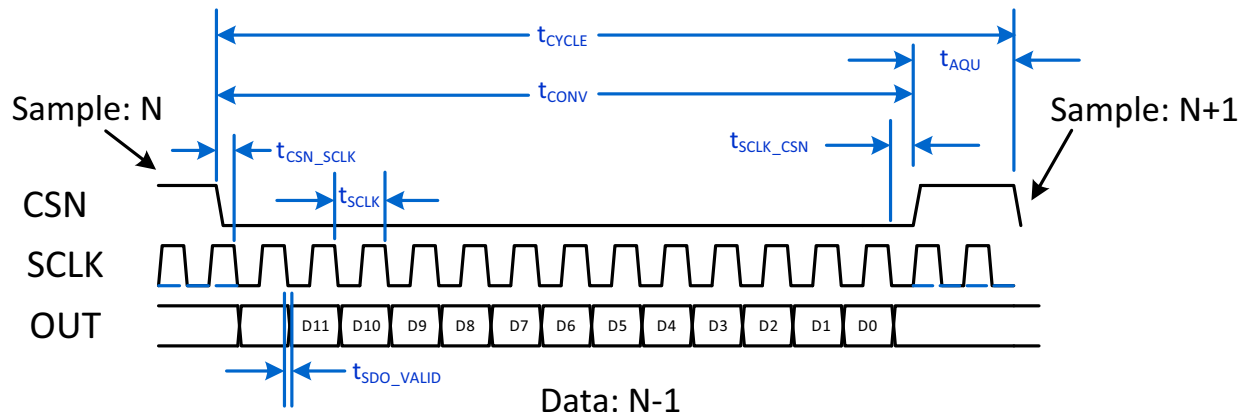
Figure 2. Serial Interface Timing
