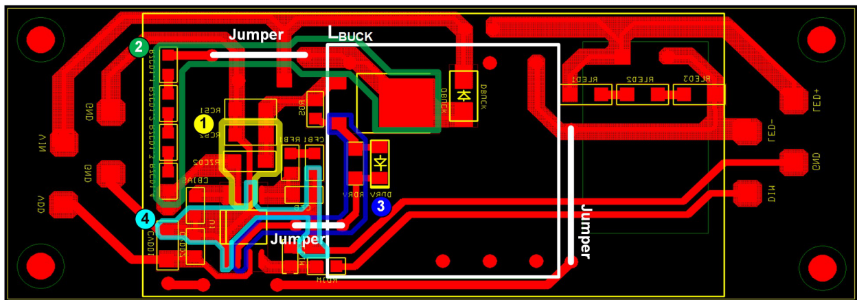
Figure 15. Layout Guidance
