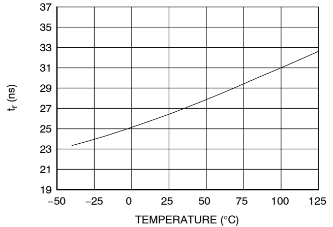
Figure 26. t_r vs. Temperature
