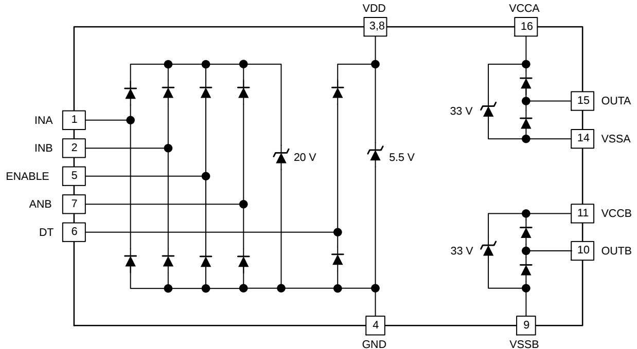
Figure 20. ESD Structure
