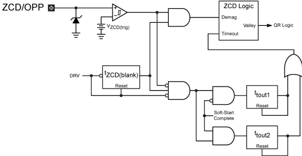
Figure 14. Valley Timeout Circuitry
