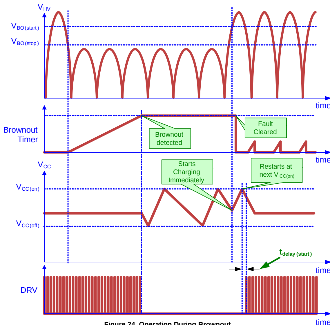
Figure 24. Operation During Brownout
