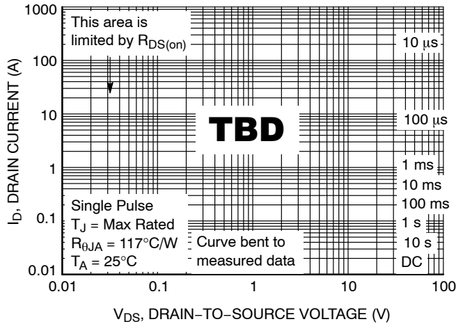
Figure 6. Highside FET Forward Biased Safe Operating Area
