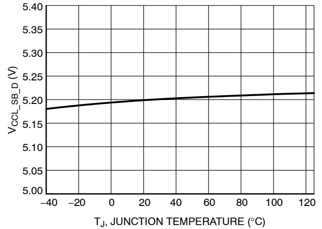
Figure 47. VCCH Current Deactivation Threshold V_{CCH\_SB\_D} = 5.2 V
