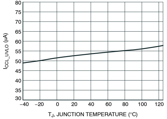
Figure 15. VCCL Current Consumption Below UVLO, V_{CCCL} = V_{OCLOFF} - 0.1 V
