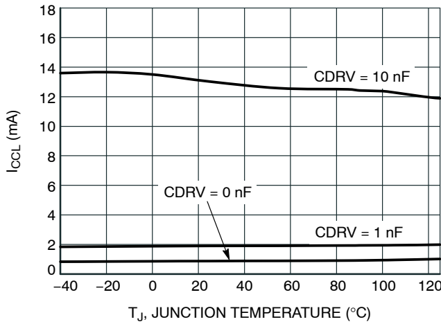
Figure 18. VCCL Current Consumption for 10 V Driver, V_{CS} = -1 to 4 V, f_{CS} = 100 kHz, V_{OCL} = 12 V
