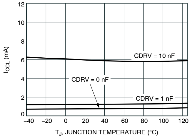
Figure 19. VCCL Current Consumption for 5 V Driver, V_{CS} = -1 to 4 V, f_{CS} = 100 kHz, V_{OCL} = 12 V
