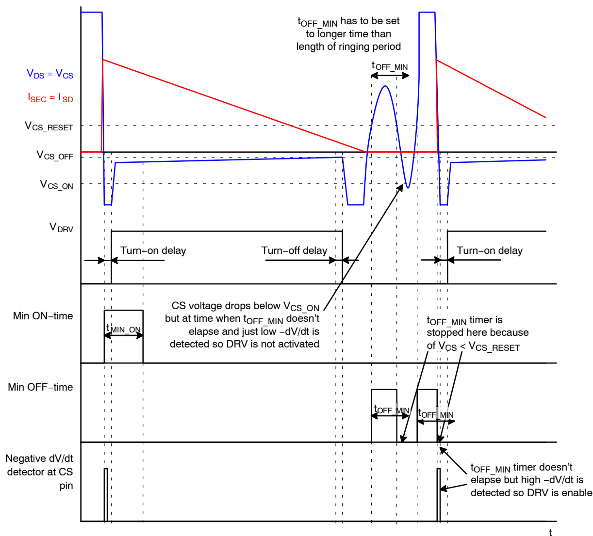
Figure 65. Situation with Enabled -dV/dt Detection
