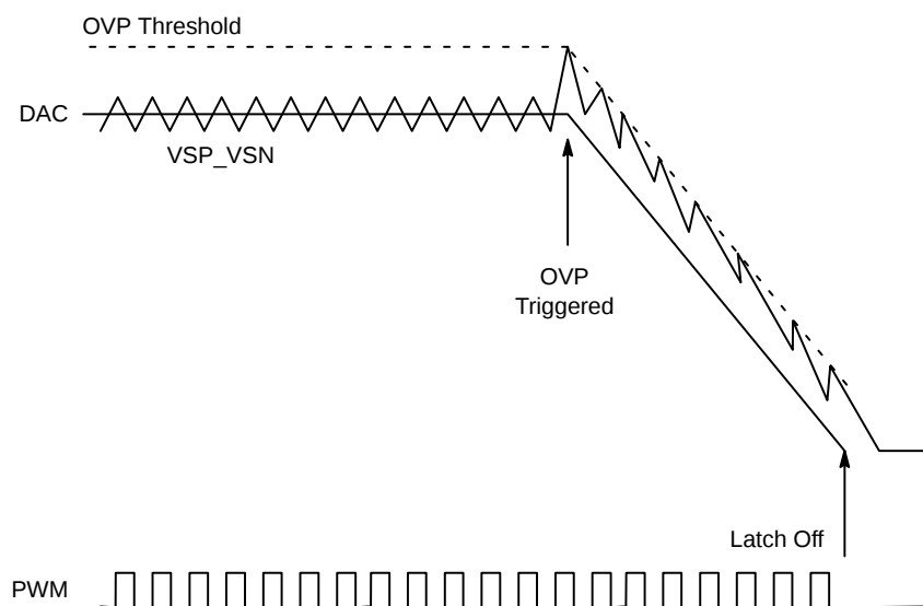
Figure 26. OVP during Normal Operation Mode
