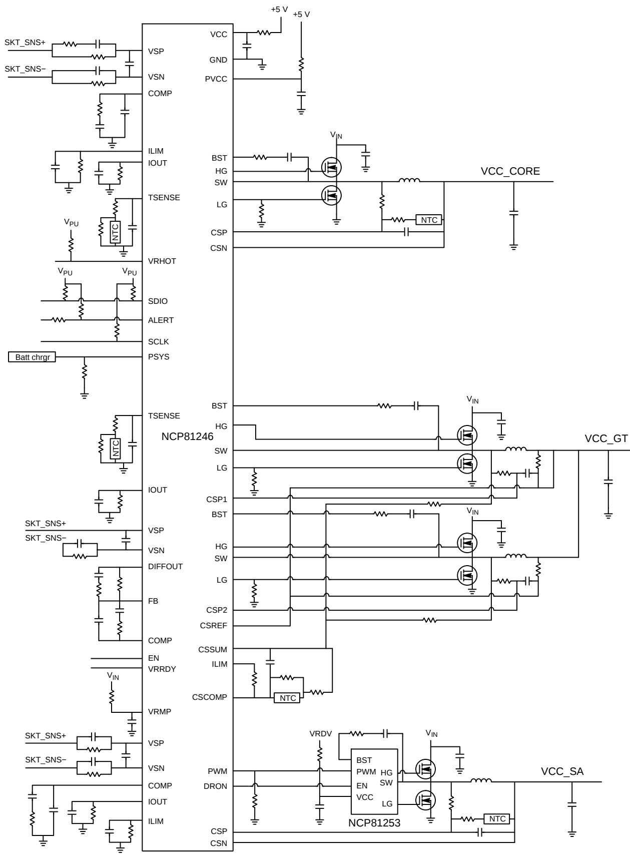
Figure 1. Application Schematic
