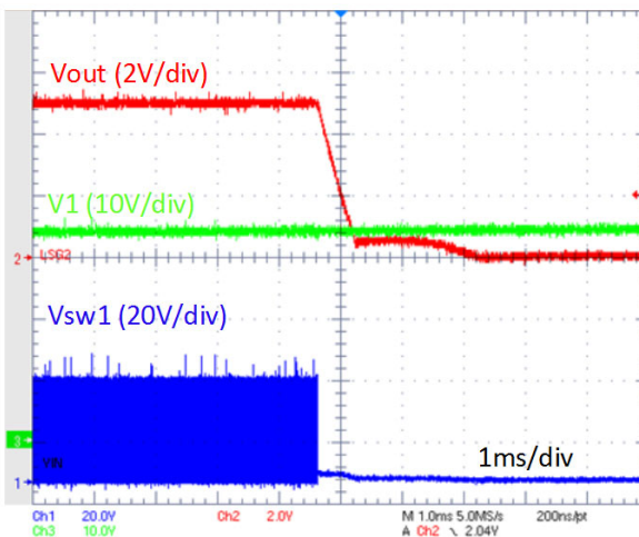
Figure 22. OVP Waveform
