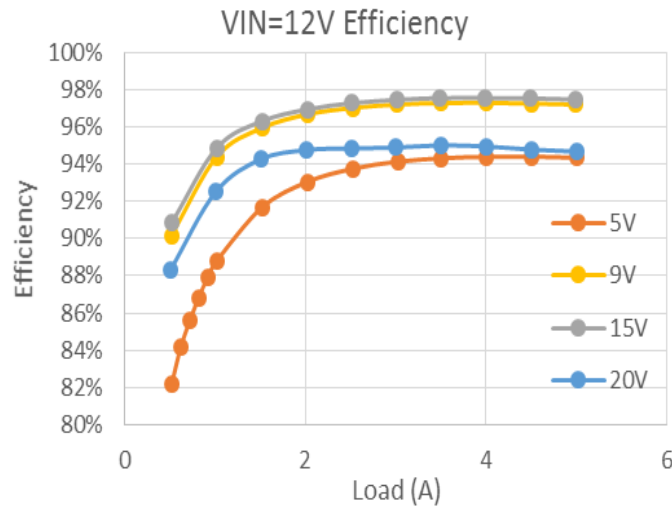
Figure 26. Efficiency vs. Load (MOSFET part number is NTMFS4C10N)
