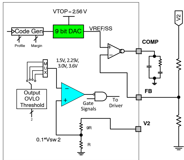
Figure 32. Output OVLO
