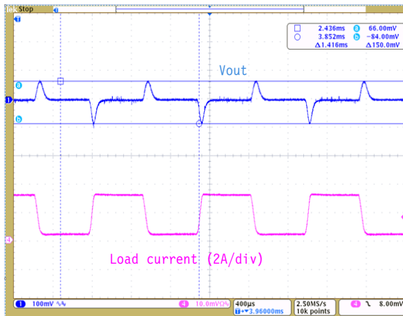
Figure 18. 5 V Load Step
