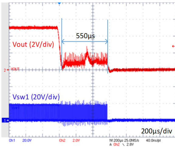
Figure 20. OCP Cycle-by-Cycle Waveform
