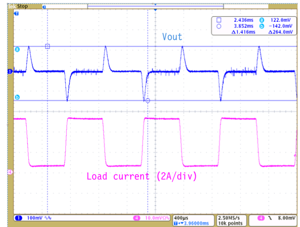
Figure 19. 20 V Load Step
