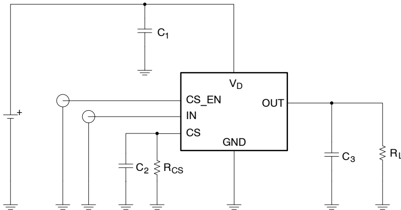
Figure 38. EMC Capacitors Placement
