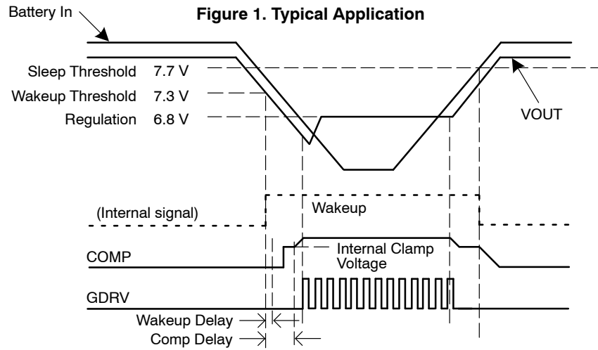
Figure 2. Functional Waveforms
