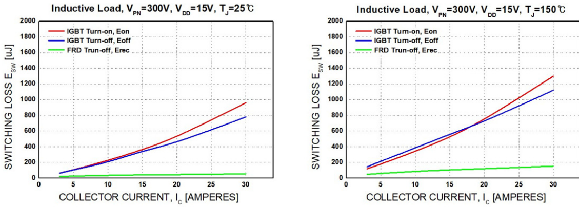
Figure 6. Switching Loss Characteristics
