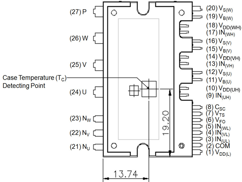
Figure 2. Top View
