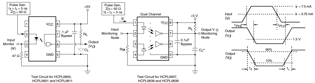
Figure 22. Test Circuit and Waveforms for t_{PLH} , t_{PHL} , t_r and t_f
