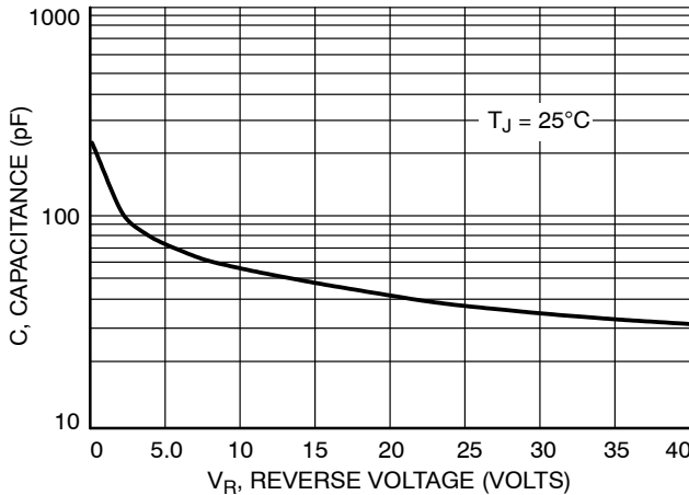
Figure 7. Capacitance
