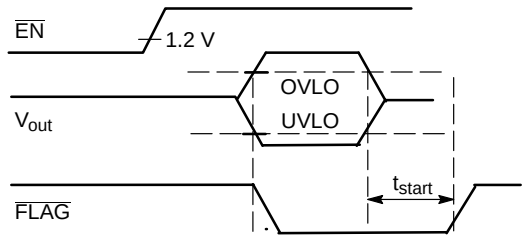
Figure 6. \overline{\text{FLAG}} Response with \overline{\text{EN}} = 1
