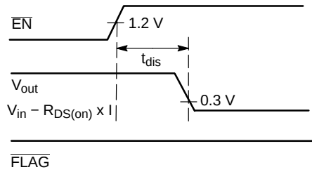
Figure 5. Disable on \overline{\text{EN}} = 1
