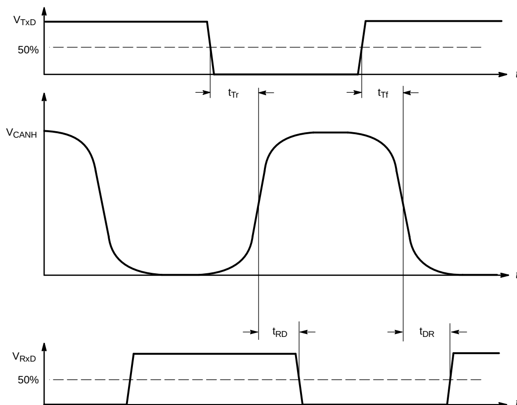
Figure 6. Input/Output Timing
