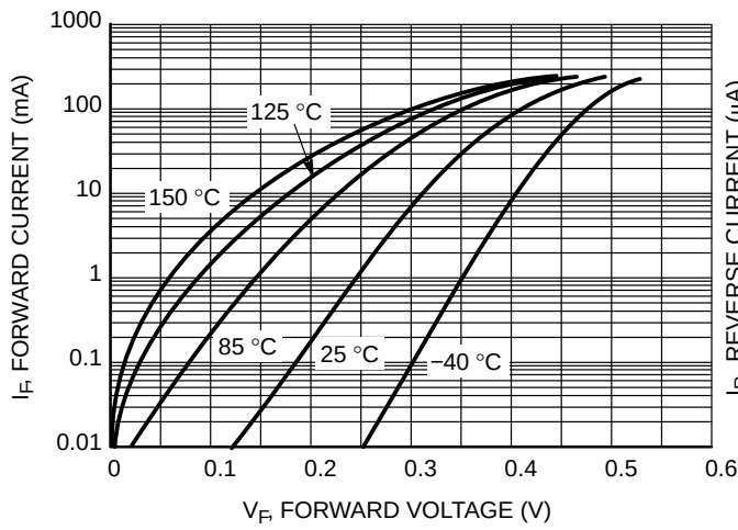
Figure 2. Forward Voltage
