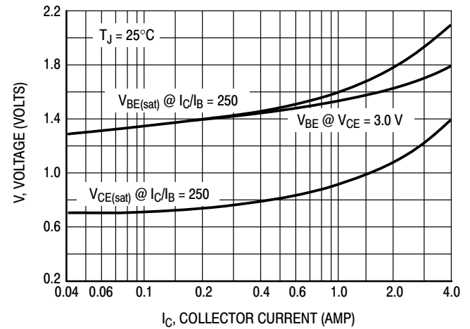
Figure 11. "On" Voltages
