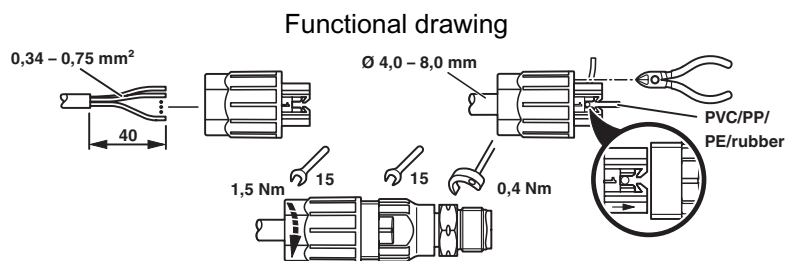
Schematic diagram
