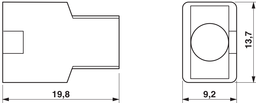
RJ45 bending protection sleeve
