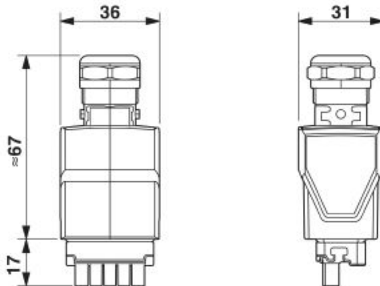
Dimensional drawing
