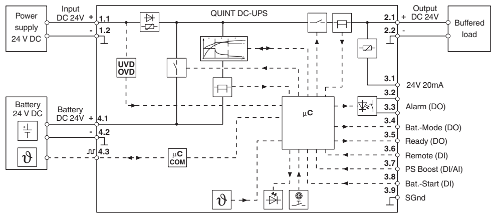
Block diagram
