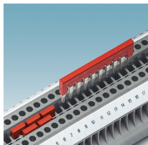
Plug-in bridge, pitch: 6.2 mm, width: 308.3 mm, number of positions: 50, color: red
