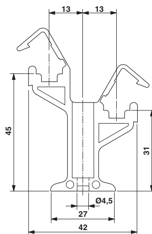
Dimensioned drawing
