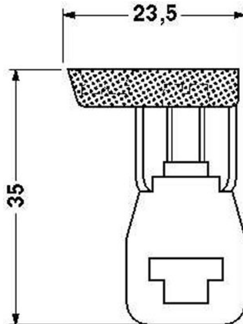
Dimensioned drawing
