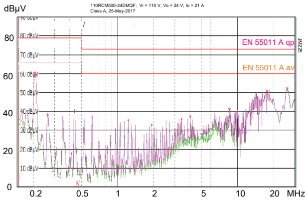
Fig. 9a 110RCM500-24: Typ. conducted disturbances at the input ( V_i = 110 V, I_{i\text{ nom}} , resistive load, quasi peak and average).
